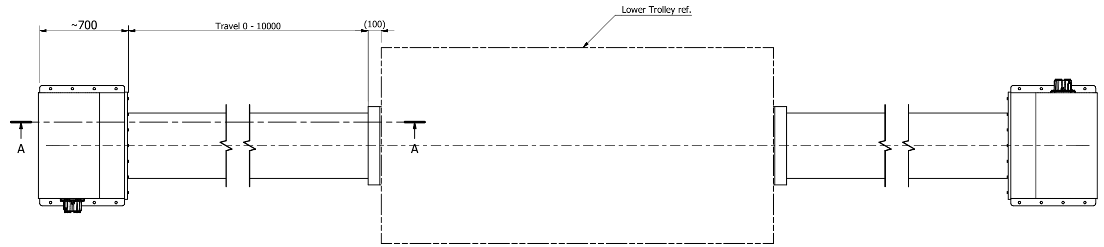
PLAN VIEW ( 1:20 )
